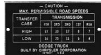
#16 Early Power Wagon Road Speed
