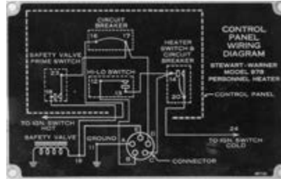
#62 (Good Used) Stewart • Warner 978 Personnel Heater Control Panel Wiring Diagram
